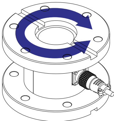
Load direction
