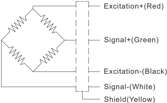
Wiring Code@Compression
